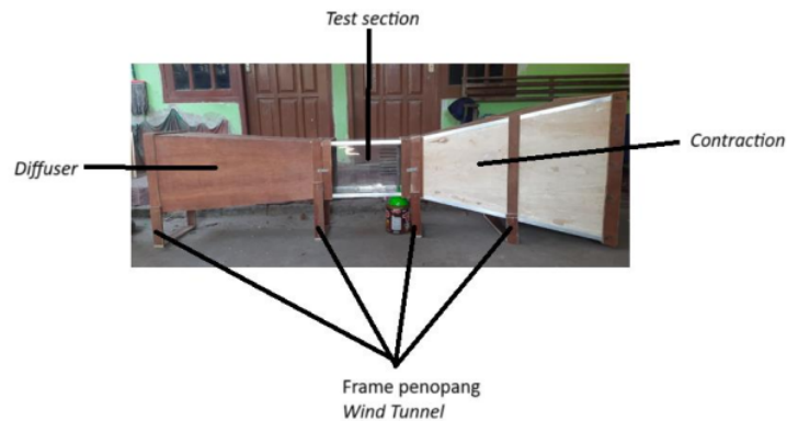
Gambar 13. Purwarupa wind tunnel
