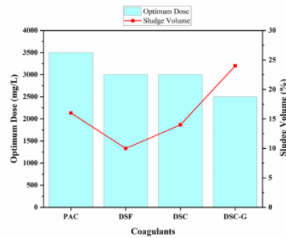
Figure 6: Comparison of optimum dose for PAC (poly aluminum chloride), DSF (durian skin flour), DSC (durian skin cellulose), and DSC-G (durian skin cellulose crosslinked with glutaraldehyde) in terms of contaminant removal efficiencies and sludge volume proportion of APSME
