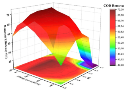
Figure 8: Interaction effects of mixing speed and pH on removal efficiency of DSC-G in terms of COD parameter in the treatment of APSME
