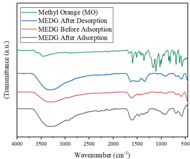
Fig. 16. IR spectra of MEDG after and before adsorption in the reusable stage.
