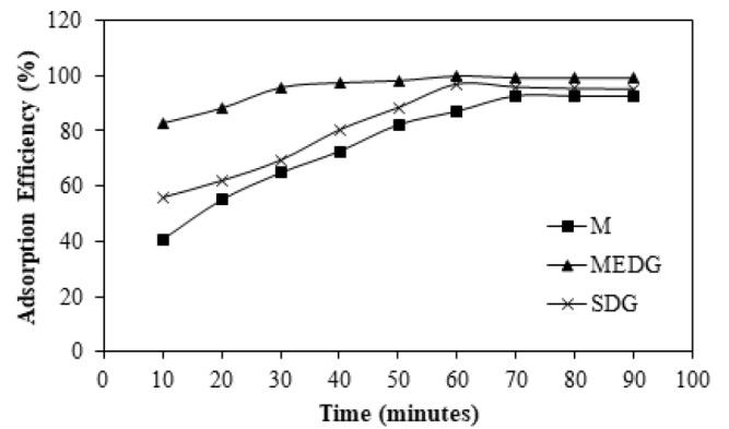
Fig. 9. Determination of the optimum contact time for adsorption.
