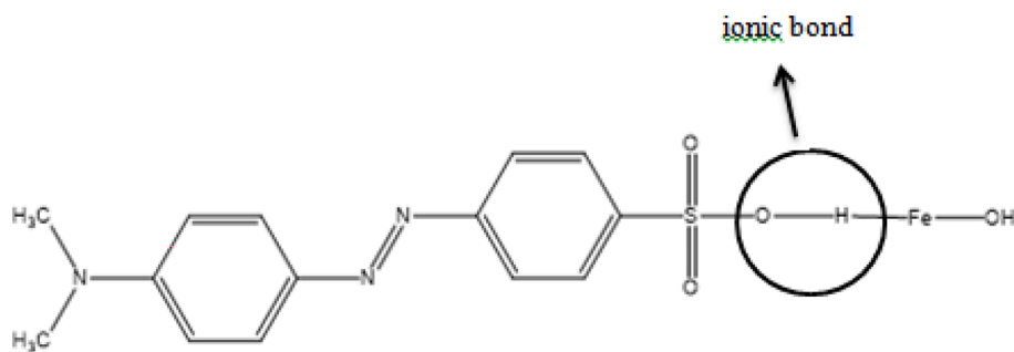
Fig. 11. The bond between M compound and MO.
