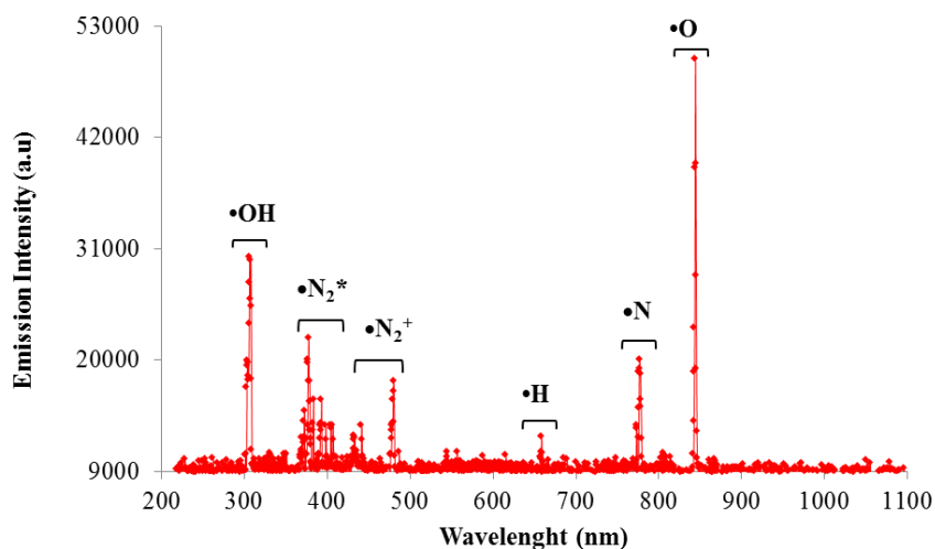
Figure 5: Radical Emission Intensity With Air Injection Flowrate 0.8 L.min -1
