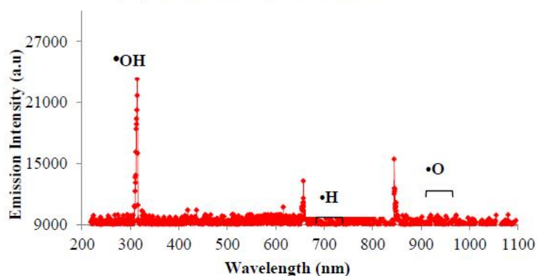
Figure 4: Radical Emission Intensity Without Air Injection
