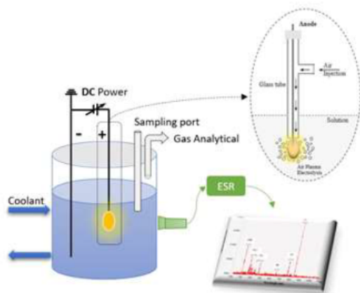
Figure 1: Experiment Apparatus
