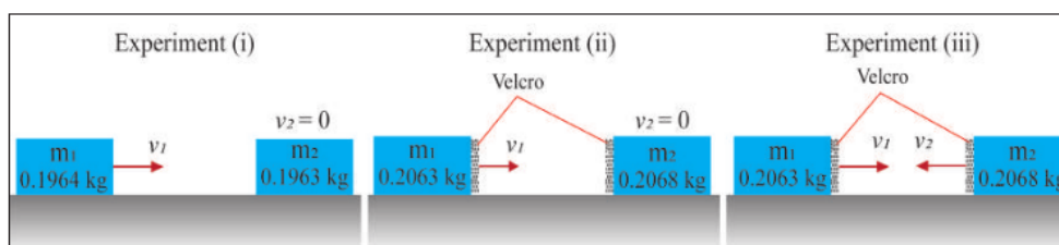
Fig. 1. Three types of collision experiments.
