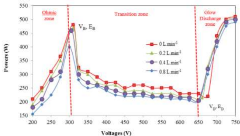
Figure 2: Voltage-Power Characterization at Different Air Injection Flow Rates
