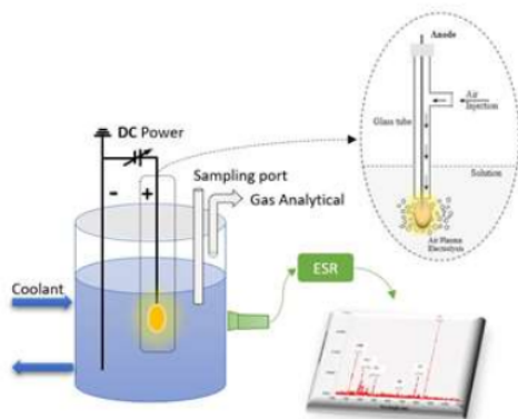
Figure 1: Experiment Apparatus
