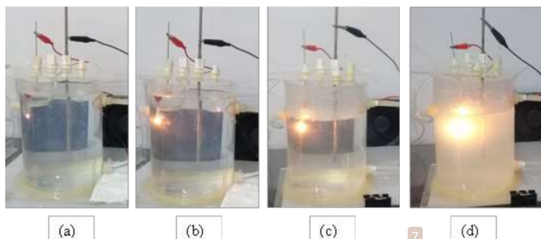
Figure 3: Plasma on Variation of Air Injection Flow Rate (a) 0 L.min -1 , (b) 0.2 L.min -1 , (c) 0.4 L.min -1 and (d) 0.8 L.min -1
