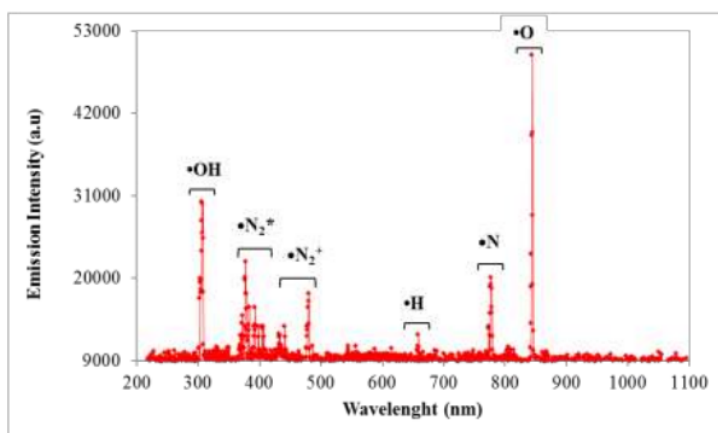
Figure 5: Radical Emission Intensity With Air Injection Flowrate 0.8 L.min -1
