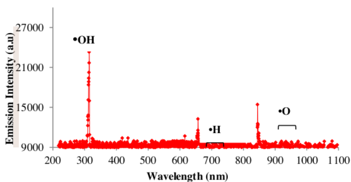
Figure 4: Radical Emission Intensity Without Air Injection
