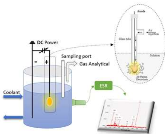
Figure 1: Experiment Apparatus
