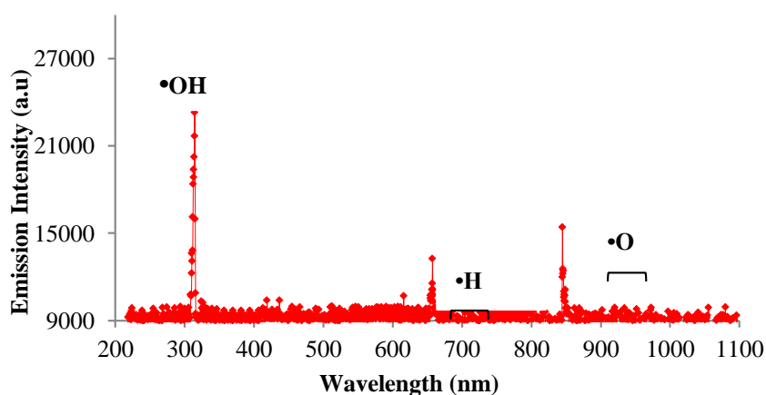
Figure 4: Radical Emission Intensity Without Air Injection
