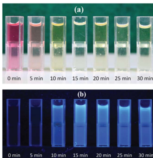
Figure 1. Dragon fruit peel extract irradiated by microwave in: (a) day light and (b) UV light.
