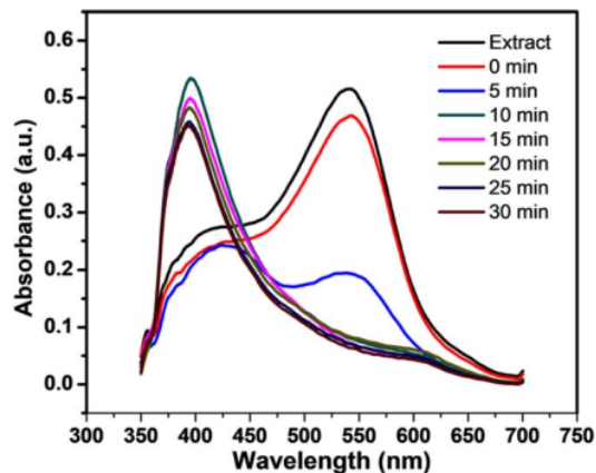
Figure 2. Absorbance spectrum of the obtained dragon fruit peel extract irradiated by microwave.
