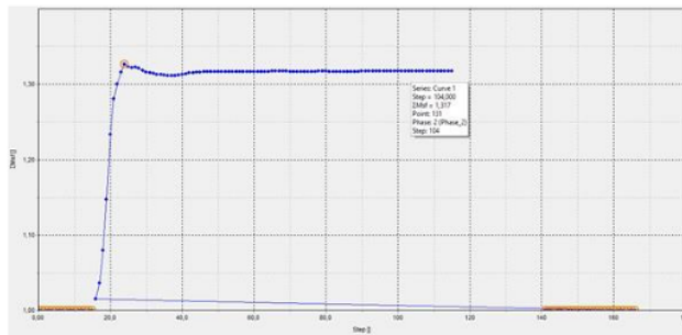
Figure 16. SF in soil with infiltration condition.
