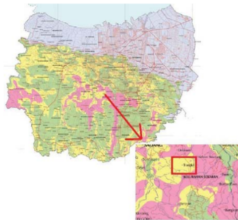
Figure 1. Location of study area [15].
