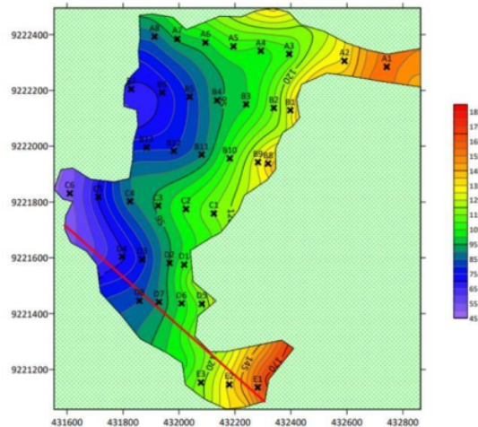
Figure 3. Topographic map of Conservation Park.
