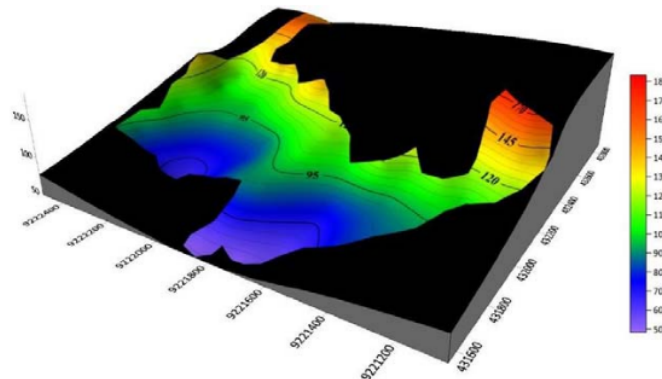
Figure 4. 3D Topographic map of Conservation Park.
