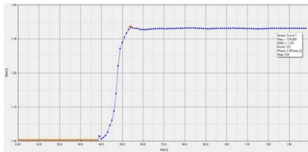
Figure 15. SF in soil with groundwater condition.
