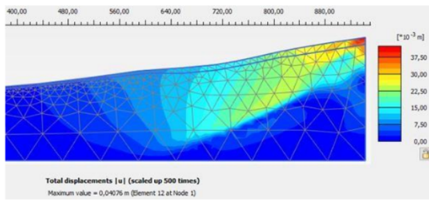
Figure 11. Soil deformation in dry conditions.
