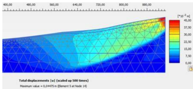
Figure 12. Soil deformation with groundwater condition
