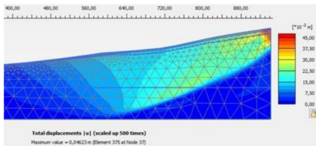
Figure 13. Soil deformation with infiltration condition.
