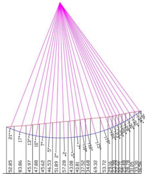
Figure 6. Trial failure surface.
