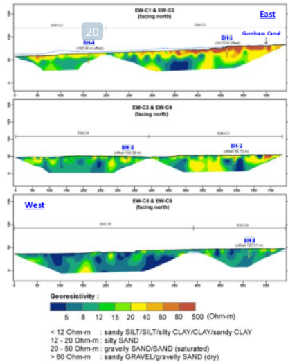
Figure 6. Results of geo-resistivity surveying along EW cross-section (Moh. Soeharto Rd.) of Petobo area during 02/2020; (up) E-segments, (middle) middle-segments, (down) W-segments.
