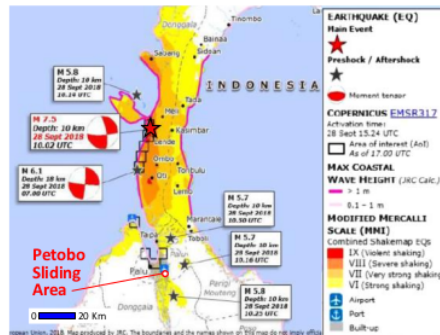
Figure 8. Foreshock, mainshock, aftershocks of 2018 Palu-Donggala EQ (GEER, 2019).
