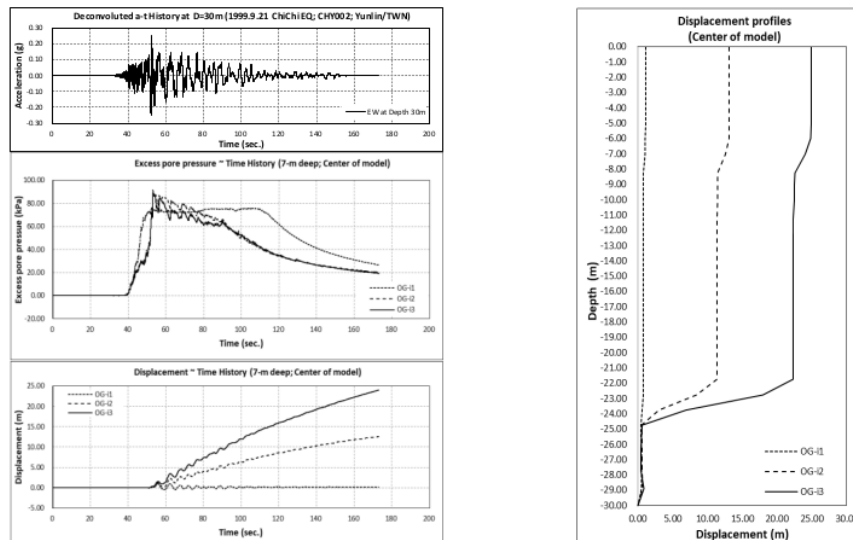
Figure 10. Verifications of liquefaction-induced flowslide behavior with different ground inclinations by OpenSeesPL (Ground surface inclination: i_1=0 / level ground, i_2=3deg. , and i_3=6deg. ).
