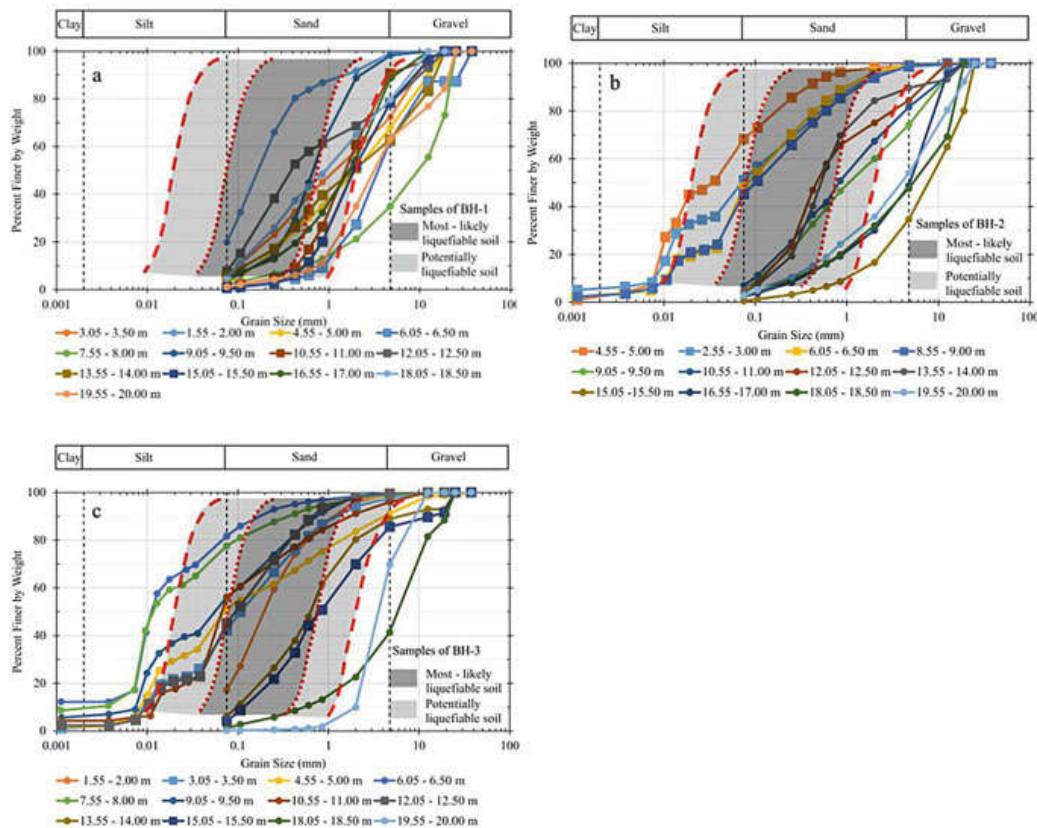
Fig. 3 Grain-size curves of SPT samples as compared with ranges of most-likely susceptible to liquefaction and potentially susceptible to liquefaction [13]
