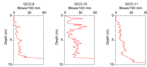
Figure 10. Results of GCO probing at Petobo site.
