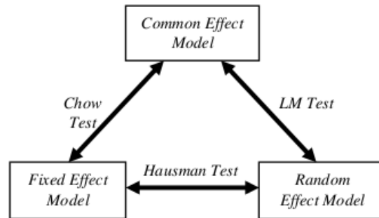
Fig 1. Selection of Best Model
