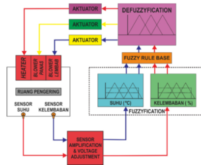
Figure 1: Dryer Block diagram.
