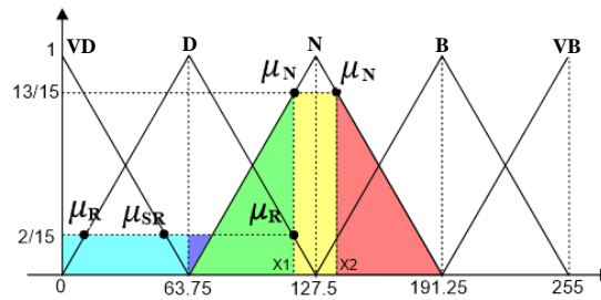
Figure 5. Composition or Aggregation Process (Max)
