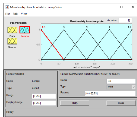
Figure 3. Lamp Membership Function Output PWM
