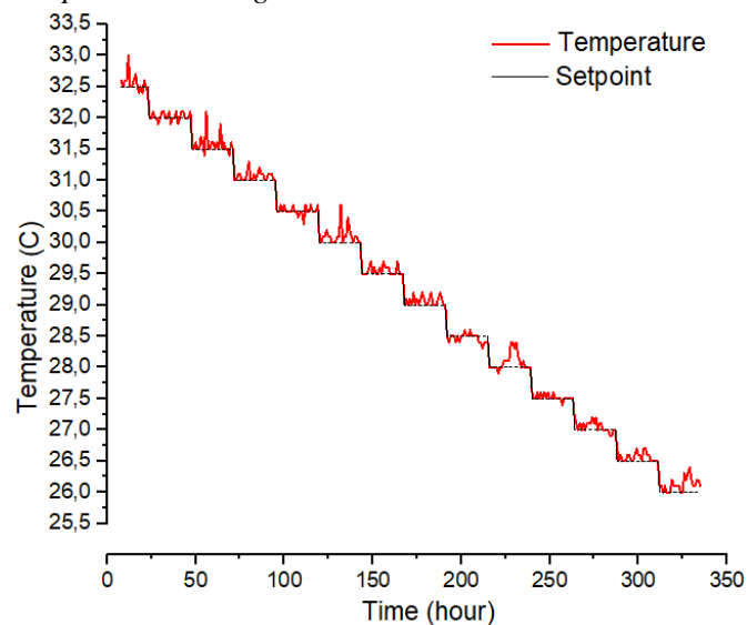
Figure 7. Graph of Temperature Changes During the Brooding Period
