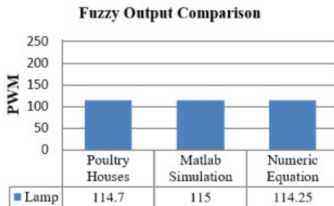
Figure 6. Comparison Graph of Mamdani's Fuzzy Output
