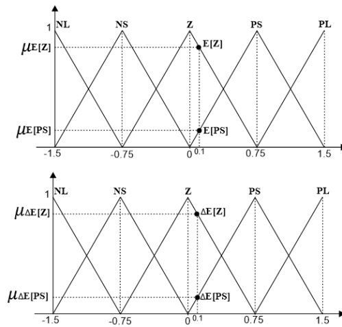
Figure 4. Evaluation of Membership function Error and Derror
