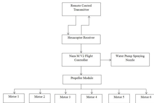
Figure 2. Planning block diagram
