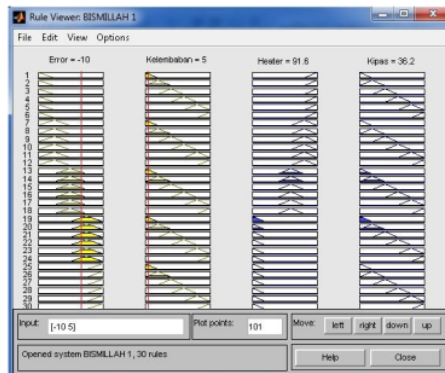
Gambar 6 Rule Viewer rancangan sistem
