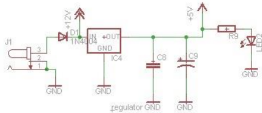
Gambar 2. Rangkaian Regulator
