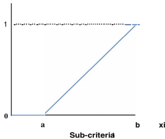
Fig. 4. Linear S-up curve model.
