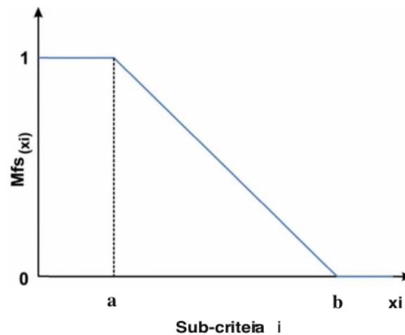
Fig. 5. Linear S-down curve model.
