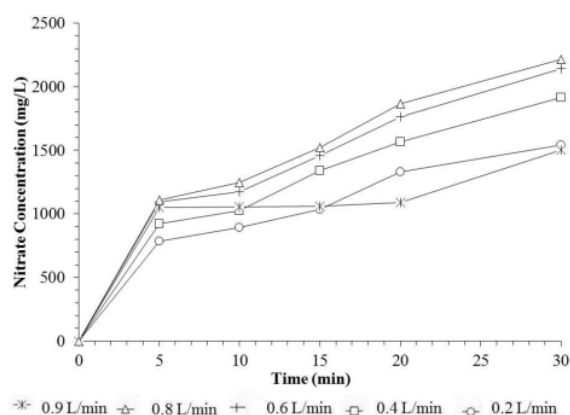
Fig. 3. Effect of air injection rate of 0.01 M K_2HPO_4 and 0.01 M K_2SO_4 on nitrate production.
