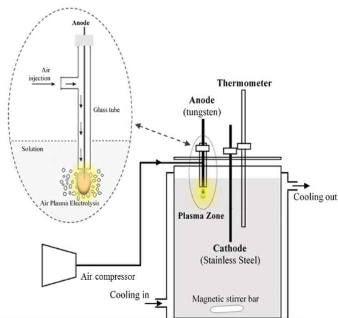
Fig. 1. Air plasma electrolysis reactor.
