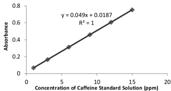
Figure 2. Calibration curve of standard caffeine solution.
