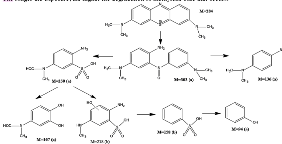
Figure 5. Photocatalytic degradation pathway of methylene blue
