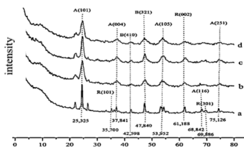
Figure 2. XRD diffractogram: a. TiO 2 ; b. NiO-TiO 2 D (300 °C H 2 -450 °C O 2 ); c. NiO-TiO 2 E (350 °C H 2 -500 °C O 2 ) and d. NiO-TiO 2 F (400 °C H 2 -550 °C O 2 )
