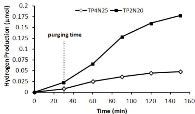
Figure 4. The hydrogen production rate of Fe-N-TiO 2 photocatalyst.
