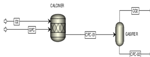
Figure 2. Simulation process for calcining coke
