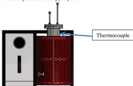
Figure 3. Thermocouple placement in the pyrolysis chamber
