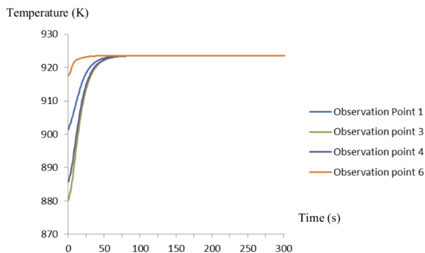
Figure 5. Temperature distribution over time across the pyrolysis chamber based on observation points after t = 4000 s
