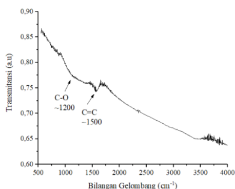
Figure 1. FTIR spectrum of graphite
