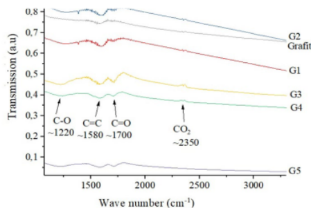
Figure 4. FTIR spectrum of graphene samples
