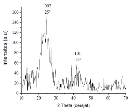
Figure 2. X-ray diffractogram of graphite
