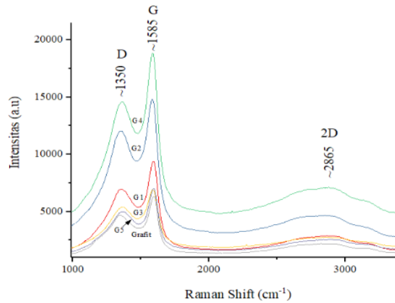
Figure 5. Raman spectroscopy results of graphene samples
