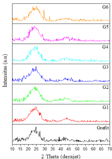
Figure 3. X-ray diffractogram for graphene samples
