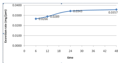
Figure 2. Flavonoid rate excretion of Carica papaya leaf.
