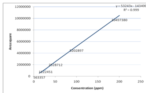
Figure 1. The standard flavonoids curve.
