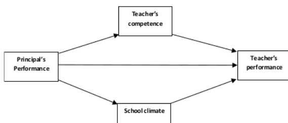
Fig. 1: Research Model
