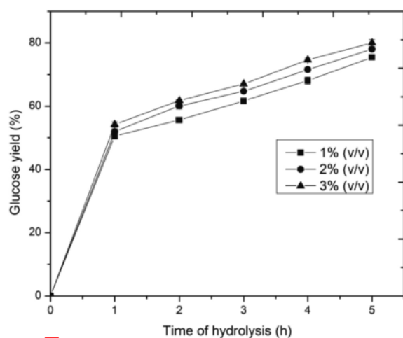
Fig. 1. The effect of glucoamylase concentration on glucose yield.
