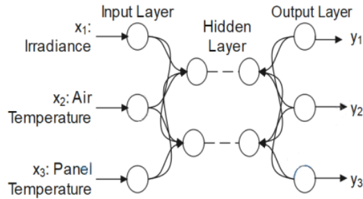
Fig. 3. The Architecture of DNN
