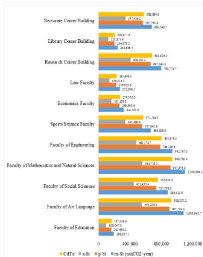
Fig 10. Rooftop photovoltaic potential and CO 2 mitigation in sub-area
