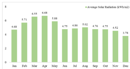
Fig 7. Average of solar irradiation prediction
