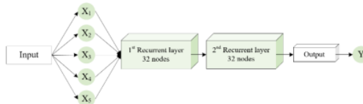
Fig 6. RNN architecture for irradiation prediction
