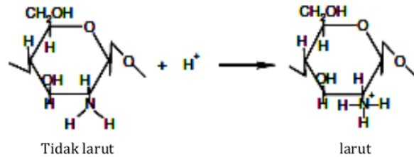
Gambar 1. Reaksi protonasi kitosan
