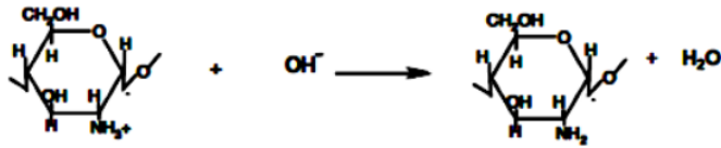
Gambar 3. Reaksi deprotonasi kitosan (Qurashi et al. 1992)
