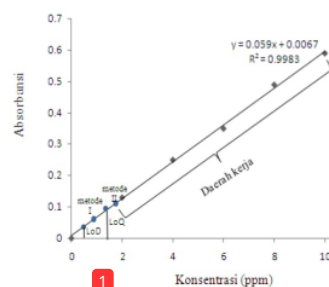
Gambar 1. Kurva kalibrasi larutan standar timbal (Pb)
