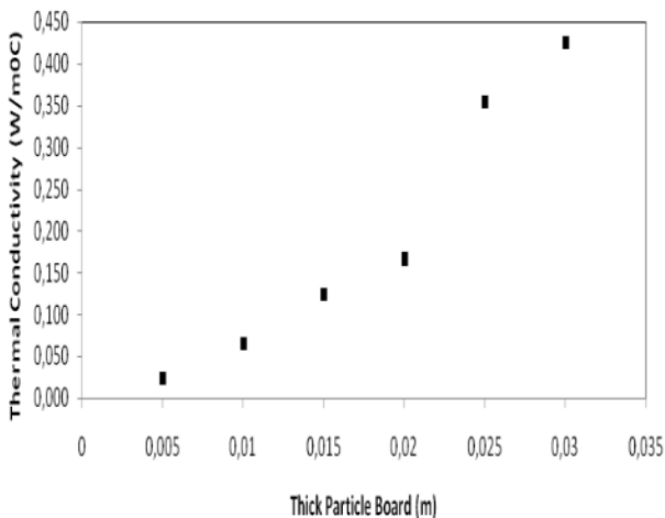
Figure 2. Particle board thickness variation graph paper on thermal conductivity.
