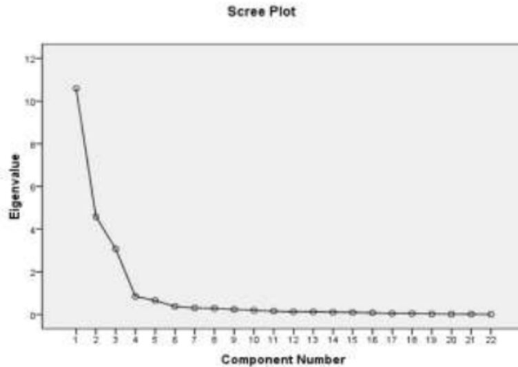
Gambar 4.1. Scree Plot
