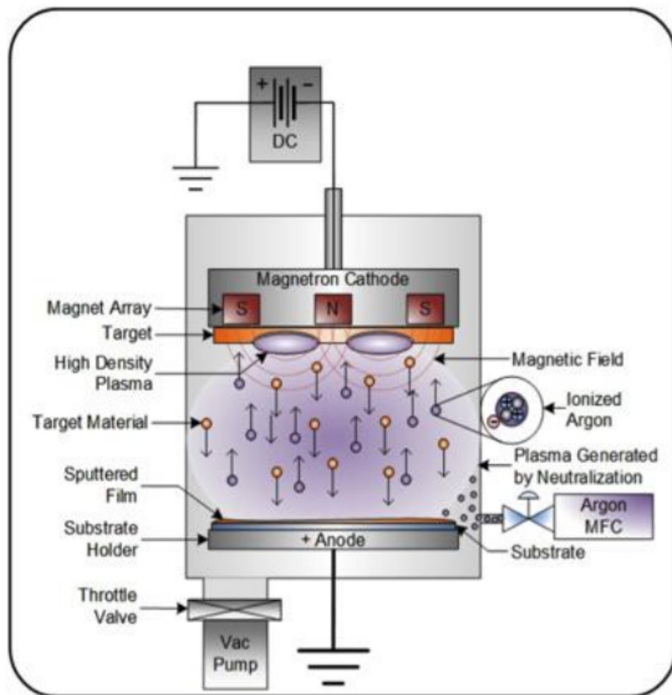
Gambar 7.13. Skema Reaksi DC Magnetron Sputtering (Hughes, 2016)
