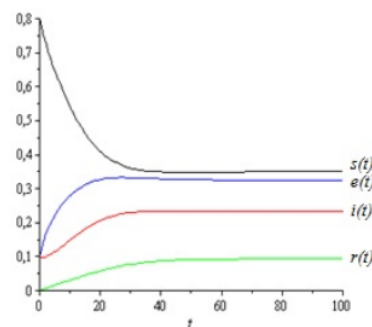
Gambar 2. Proporsi individu susceptibles s(t) , exposed e(t) , infectious i(t) , dan recovered r(t) .
