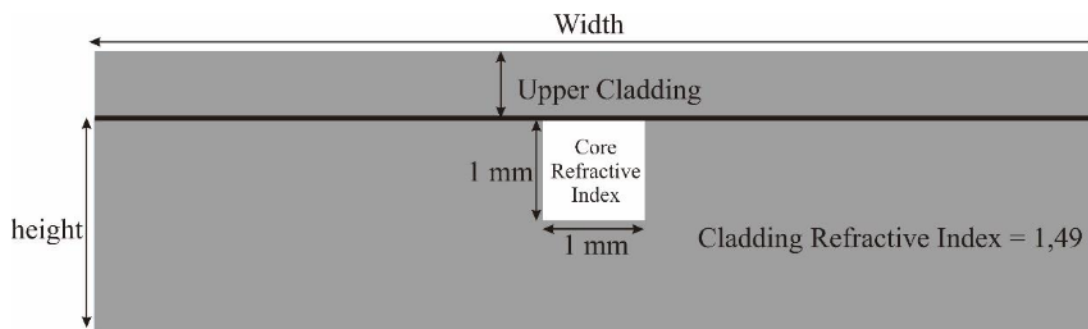
FIGURE 1. Buried waveguide parameter structure design.
