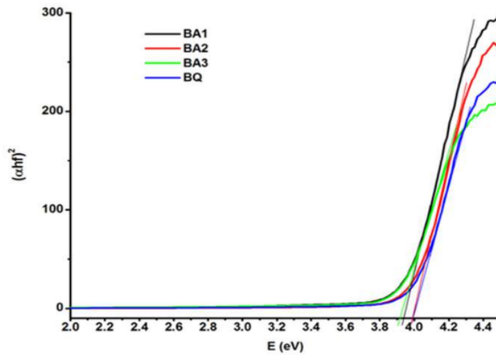
Figure 3. Tauc's plot (\alpha hf)^2 versus E (eV).
