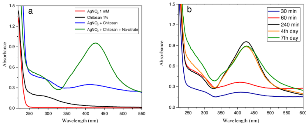
Figure 2. a) The UV-visible spectra of a) AgNPs-Ch prepared with and without Na 3 -citrate, b) The growth and stability of AgNPs-Ch
