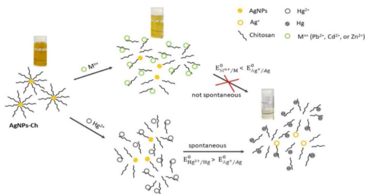
Figure 6. The proposed detection mechanism of Hg 2+ by AgNPs-Ch nanocolloid
