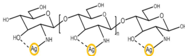
Figure 1. The amine (-NH 2 ) and hydroxyl (-OH) of chitosan covering and stabilizing AgNPs
