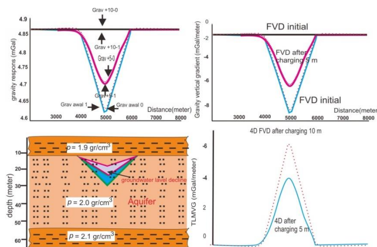
Figure 3. Response TLMVG anomaly caused by groundwater level increase
