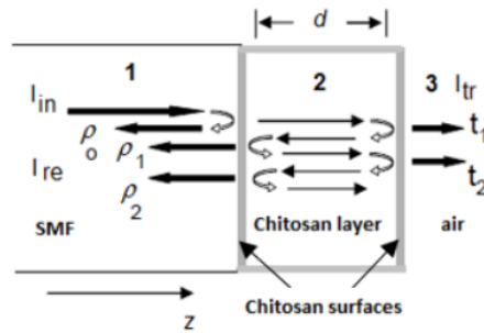
Figure 1. Chitosan layer-based FPI optical sensor
