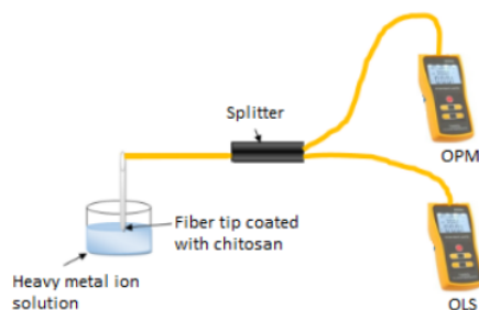
Figure 2. Characterization set up for sensitivity determination
