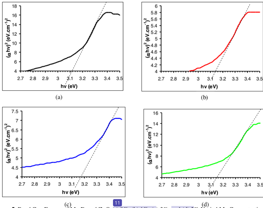
11 Figure 5. Band Gap Energy of Mg Doped ZnO (a) 0%, (b) 1%, (c) 3%, and (d) 5% Varied Mg Concentration
