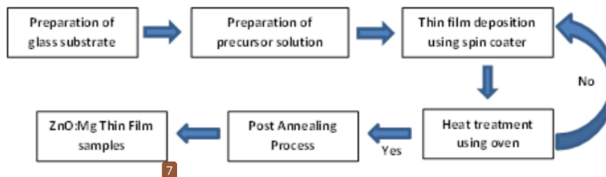
Figure 1. The Schematic of the ZnO: Mg Thin Film Grown by Using Sol-Gel Spin Coating Method
