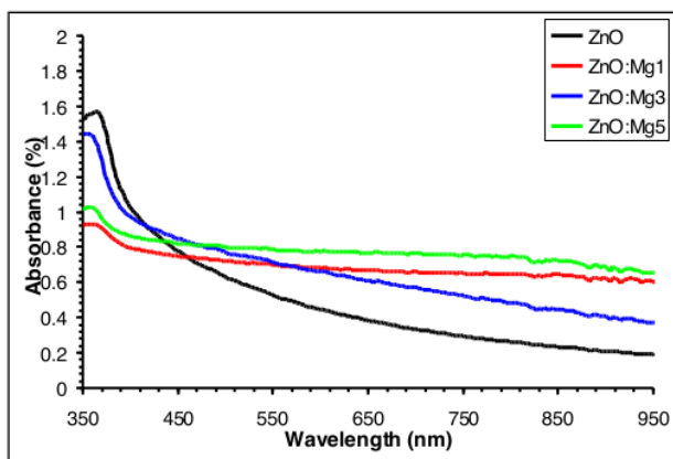
Figure 4. UV-VIS Spectra of ZnO Doping Mg Thin Film with Different Mg Concentration
