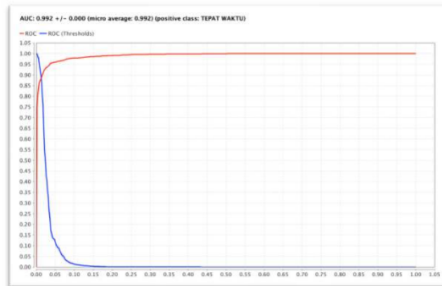
Figure 3. AUC graph
