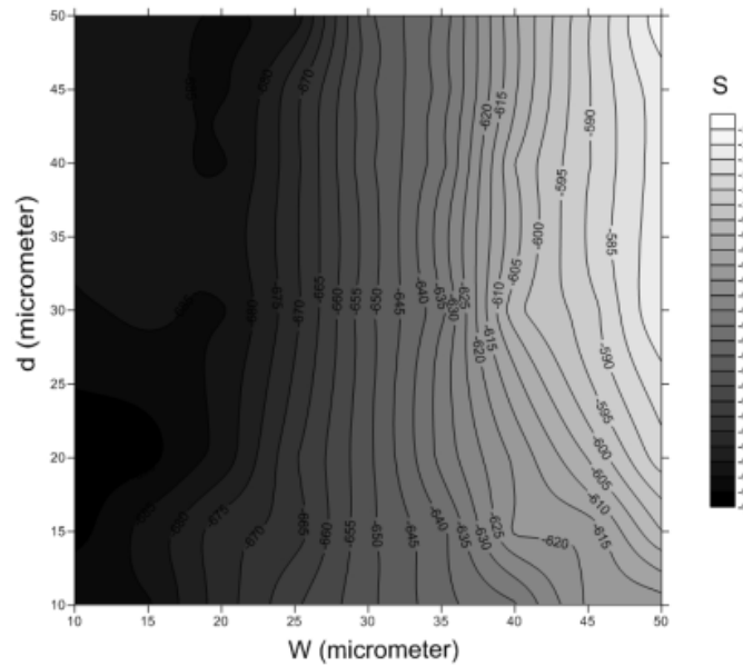
Fig. 4. Temperature sensitivity of ridge waveguide for various widths and various thicknesses.
