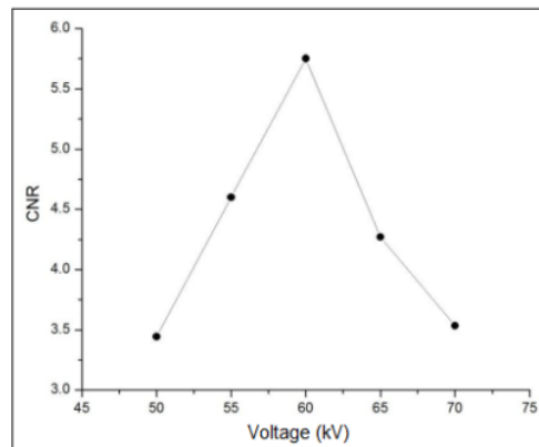
Figure 4. CNR vs. voltage for pearl oyster image.
