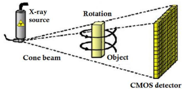
Figure 1. Schematic diagram of micro CT [9].
