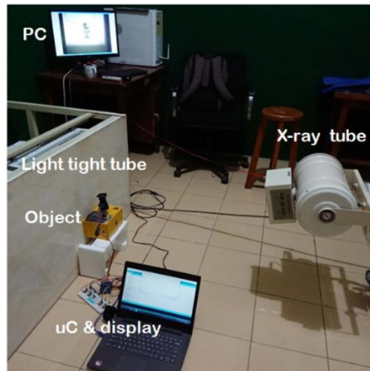
Figure 3. MicroCT acquisition system
