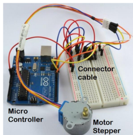
Figure 2. Stepper motor with arduino micro controller [10].
