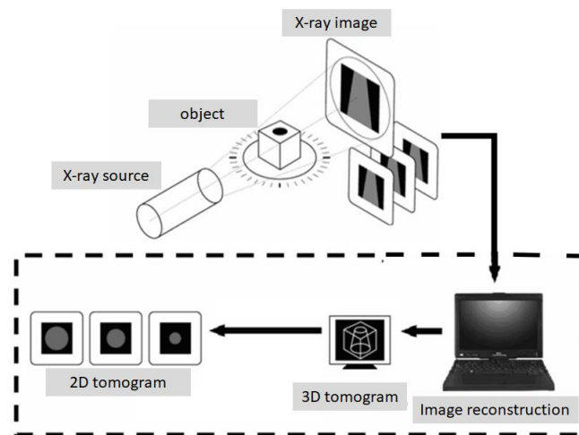
Figure 4. Simulated CT system built in this study.
