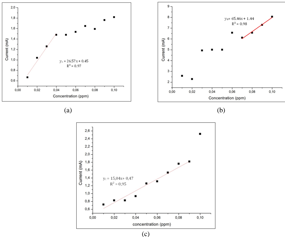
Figure 2. Current vs cadmium concentration for sensor A (a), sensor B (b) and sensor C (c)
