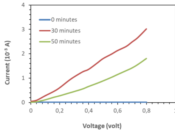
Figure 4. I-V measurement of AZO thin films.
