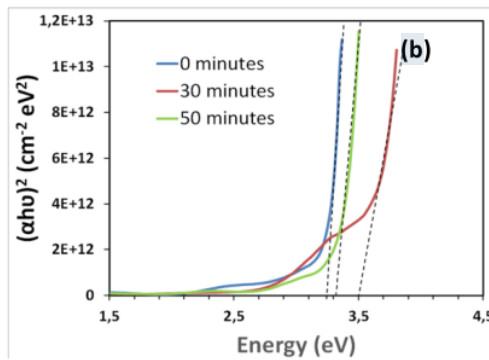
Figure 3b. The energy gap of the AZO films estimated by the extrapolation of the linear part of the (ahv)^2 versus hv plots.
